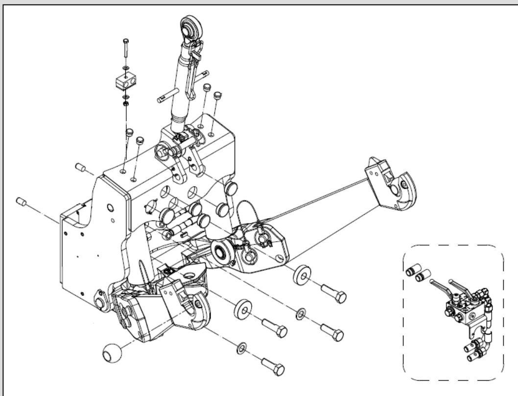
PZZ 18 kN (1410112)
